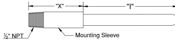
Protection tube with Mounting Sleeve (No process conn.)
