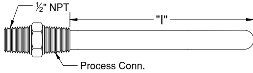
Protection tube with Double ended Hex Fitting
