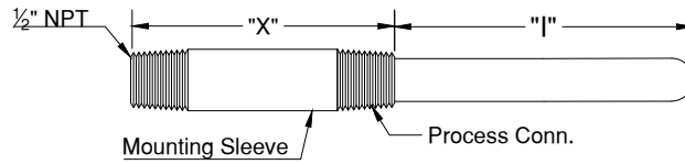
Protection tube with Mounting Sleeve and Process Connection
